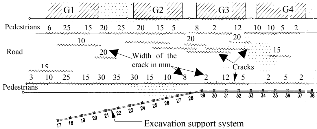
Figure 3 : Observed damages and cracks in plan after the 3 th excavation (-6.8 m).
