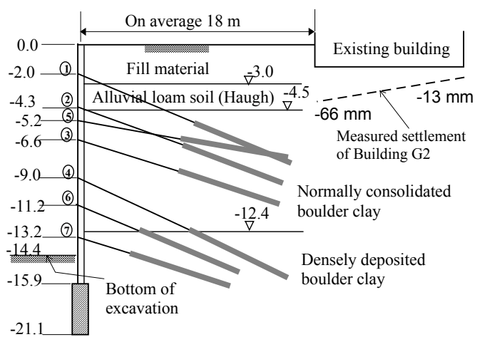
Figure 2 : Soil profile, Wall and anchor arrangements, and the measured settlement profile of the building.
