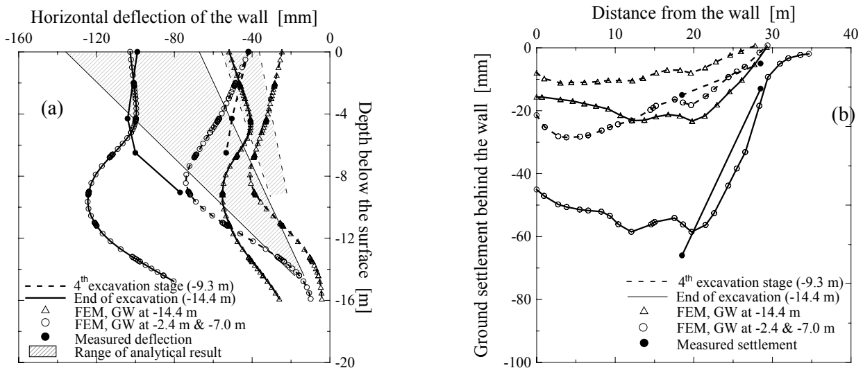
Figure 6 : a) Horizontal deflection of the wall, and b) settlement of the ground behind the wall after the 4 th excavation (-9.3 m) and full excavation (-14.4 m).
