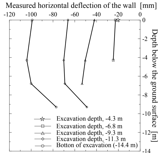
Figure 4 : Measured horizontal deflection of the wall at various construction stages.
