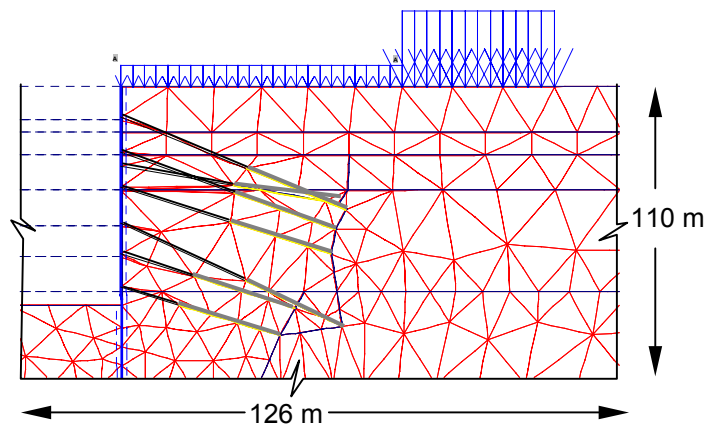
Figure 5 : Finite element mesh.
