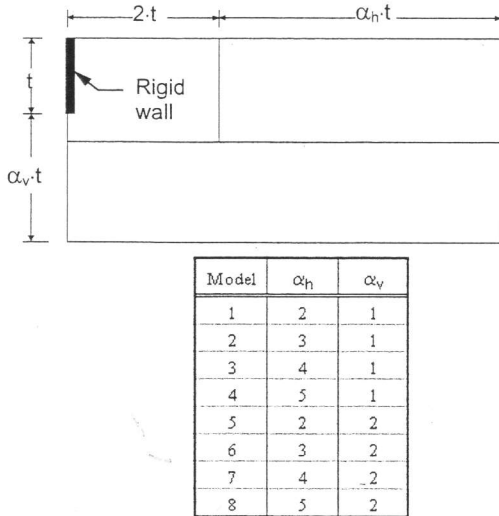
Figure 2. Model geometry selection
