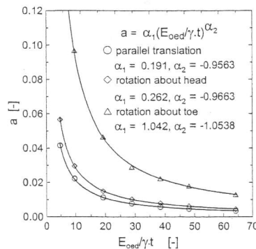
Figure 6. Relationships between the normalized constrained modulus E_{oed} and the curve constant a for t = 8 m
