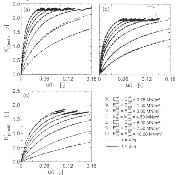
Figure 4. The mobilization of the net passive resistance: a) parallel translation, b) rotation about the head, and c) rotation about the toe
