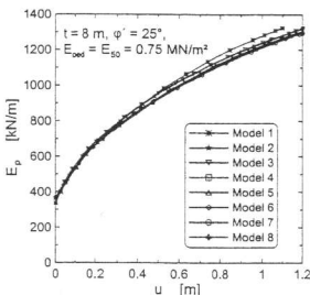
Figure 3. Mobilized passive force from different model sizes
