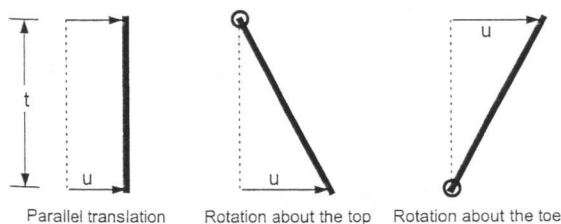
Figure 1. Types of the wall movement
