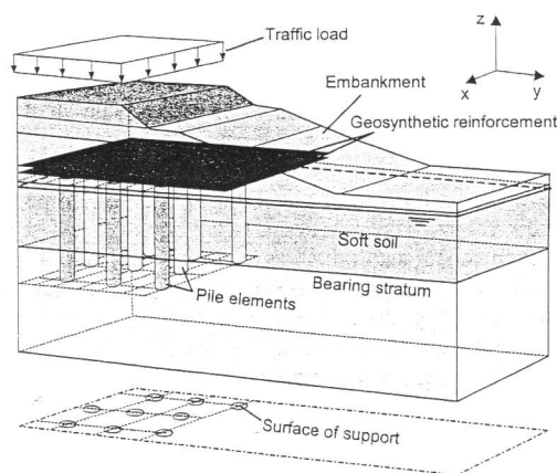
Figure 1. Geosynthetic-reinforced pile-supported embankment
